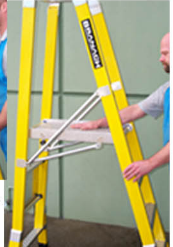
Push platform firmly down and engage hooks
